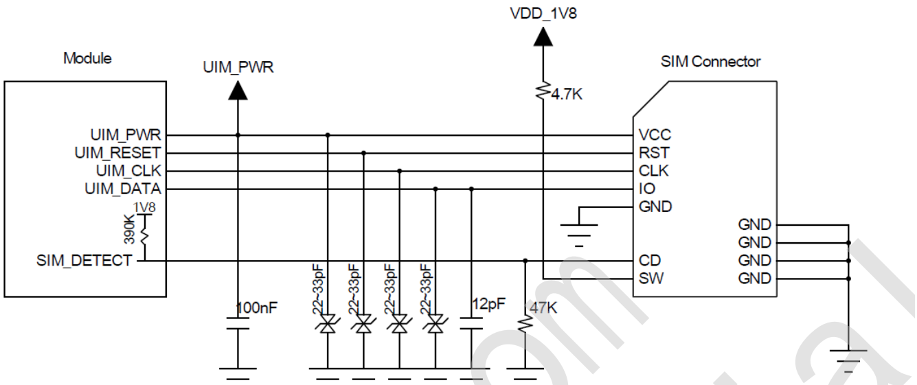
Figure 3-16 Reference circuit for N.O. SIM card slot
