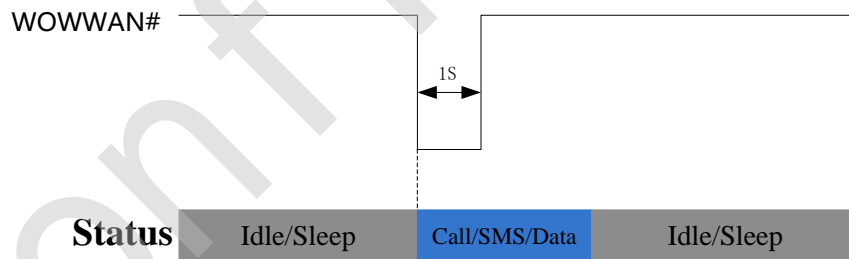
Figure 3-18 WOWWAN# timing
