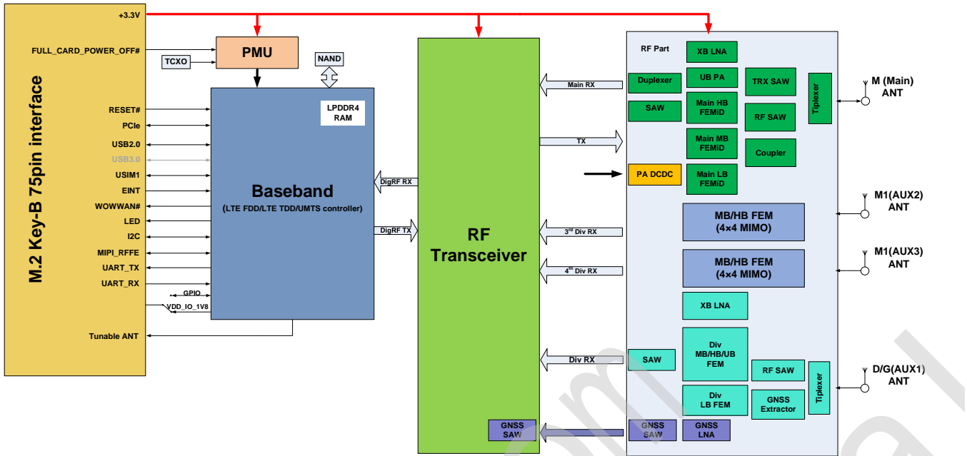
Figure 2-2 Hardware block diagram
