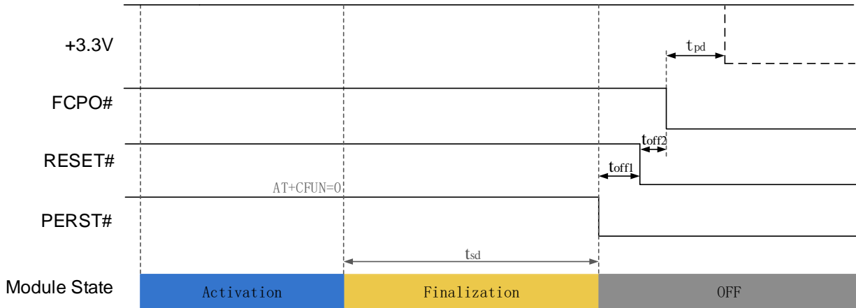
Figure 3-6 Shutdown timing control
