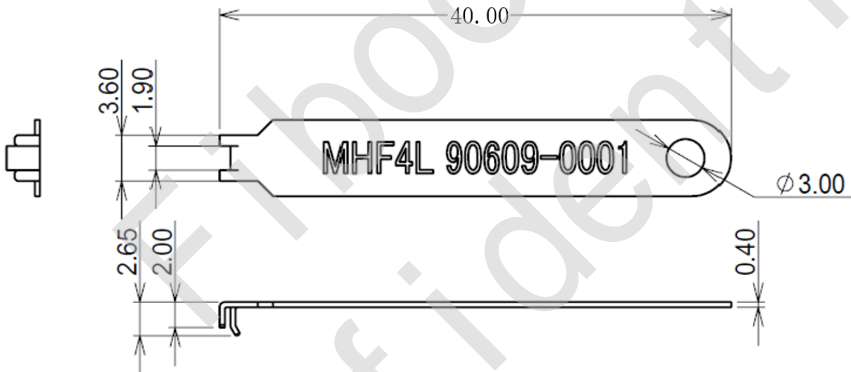
Figure 4-6 Pulling JIG
